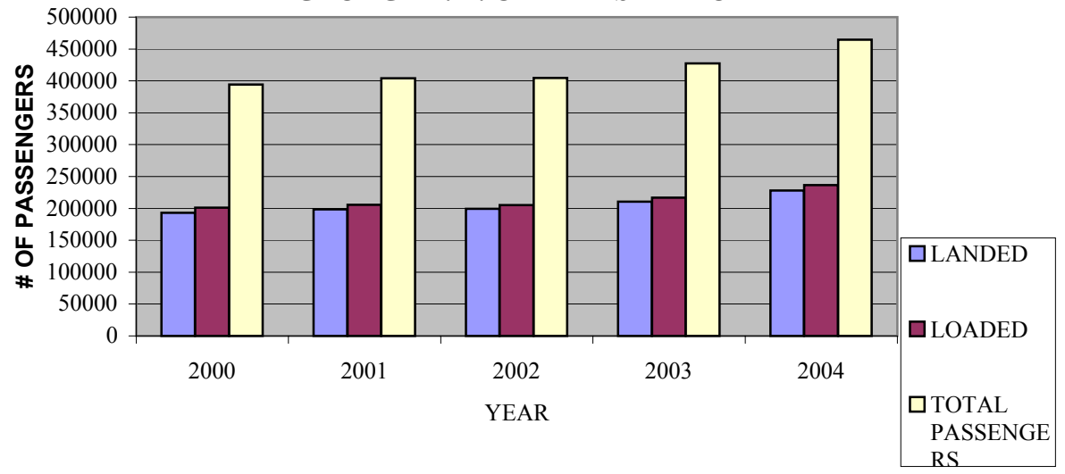
CHART 2.304 PASSENGER TRAFFIC AT GEORGE F. L. CHARLES AIRPORT
